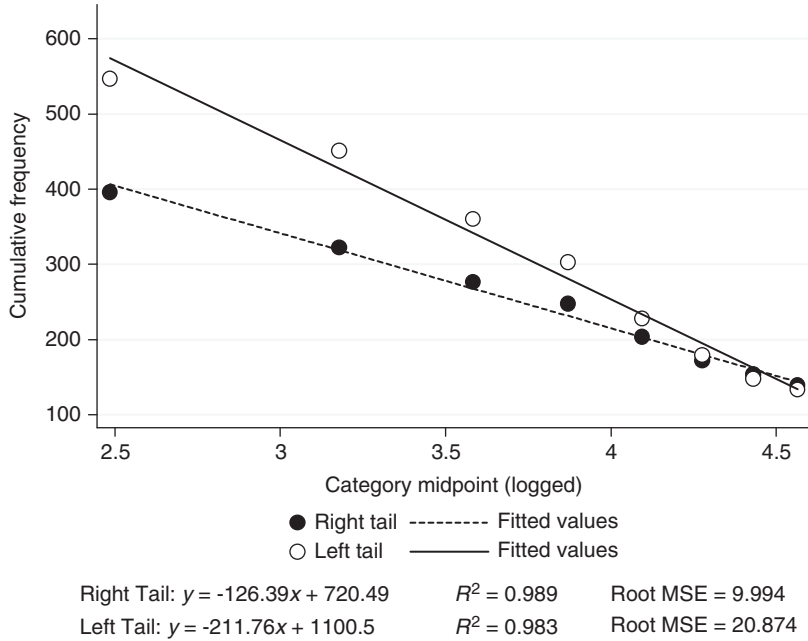
Fig. 4. Semi-log plot with a superimposed line of best fit
