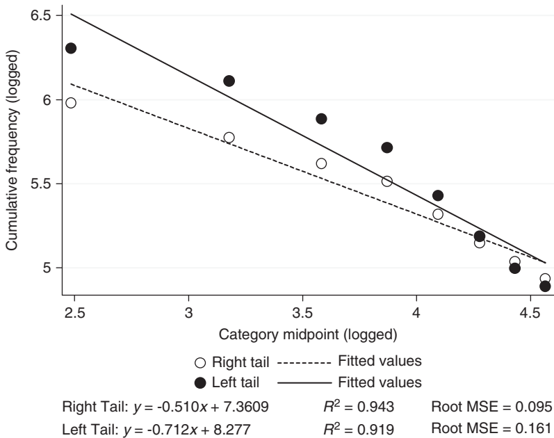
Fig. 5. Log-log plot with a superimposed line of best line
